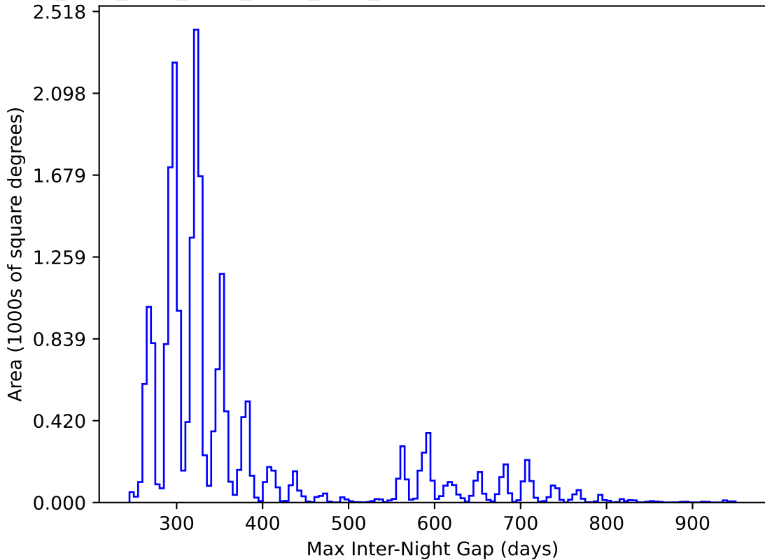
ddf_acor_sf10_lsf30_lsr50_v3.4_10yrs All sky y band: Max Inter-Night Gap
