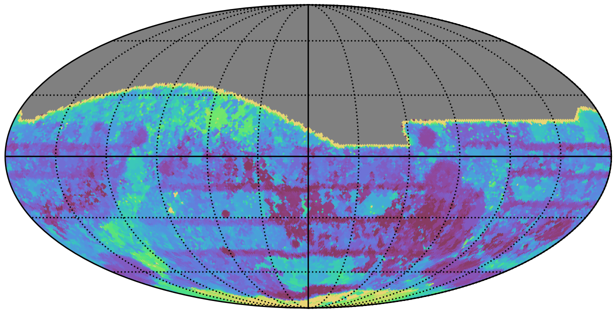
ddf_acor_sf10_lsf30_lsr50_v3.4_10yrs All sky all bands: Max Inter-Night Gap
