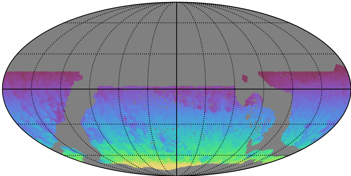
ddf_acor_sf10_lsf30_lsr50_v3.4_10yrs WFD all bands: Max HA
