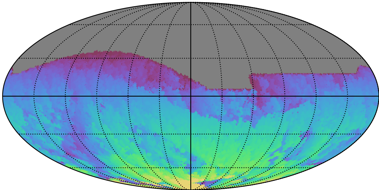
ddf_acor_sf10_lsf30_lsr50_v3.4_10yrs All sky z band: Max HA
