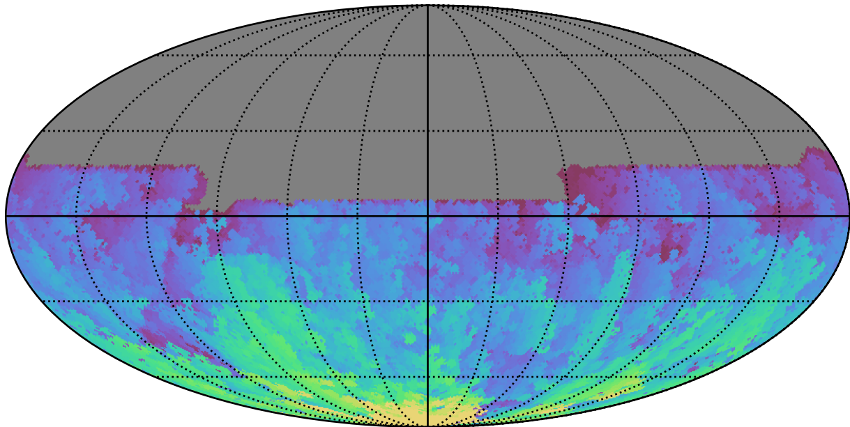
ddf_acor_sf10_lsf30_lsr50_v3.4_10yrs All sky u band: Max HA
