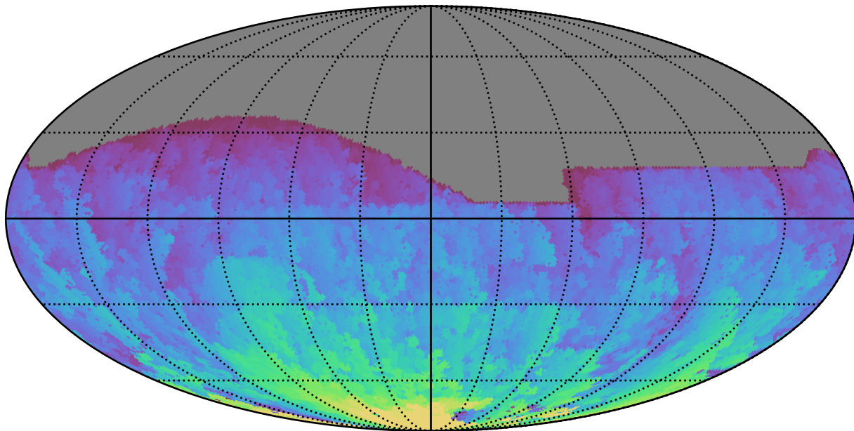
ddf_acor_sf10_lsf30_lsr50_v3.4_10yrs All sky r band: Max HA
