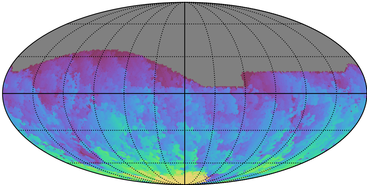
ddf_acor_sf10_lsf30_lsr50_v3.4_10yrs All sky g band: Max HA
