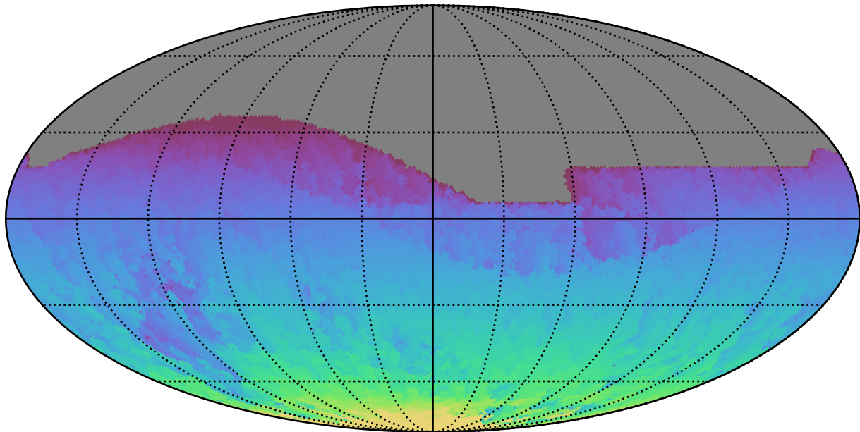
ddf_acor_sf10_lsf30_lsr50_v3.4_10yrs All sky all bands: Max HA
