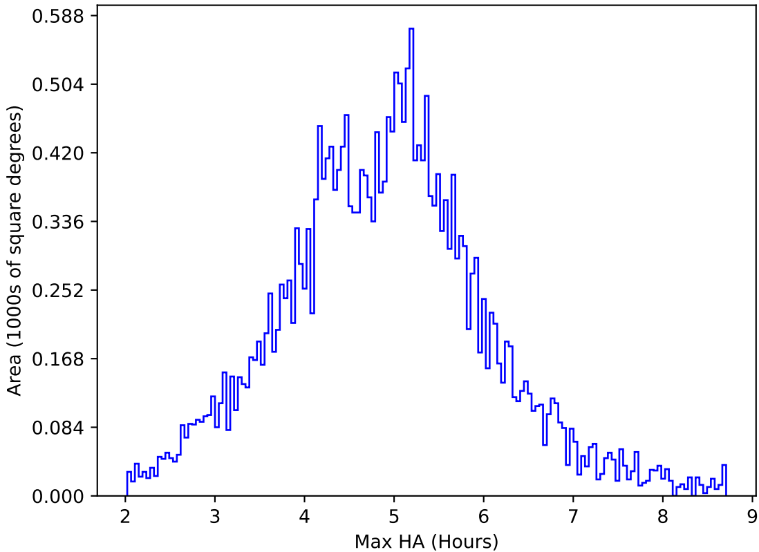
ddf_acor_sf10_lsf30_lsr50_v3.4_10yrs All sky all bands: Max HA
