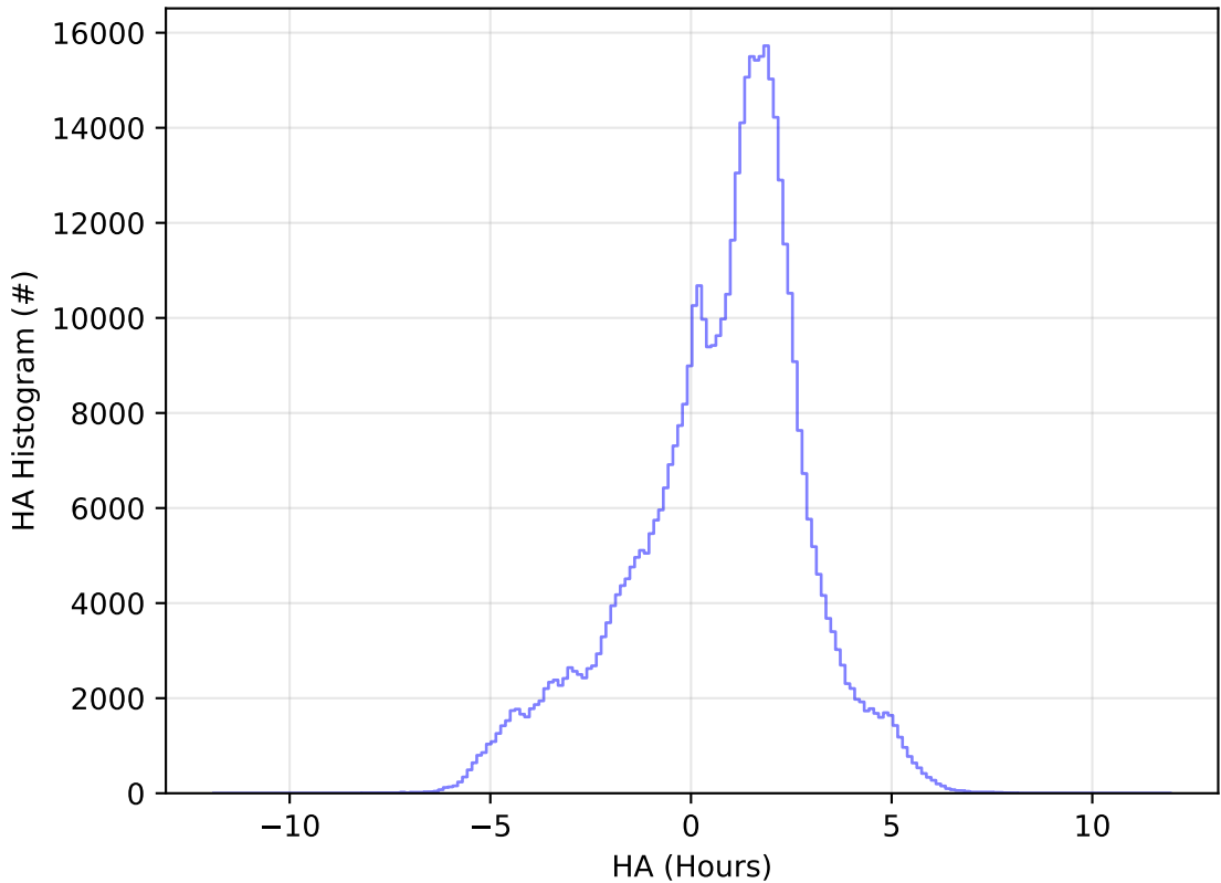
ddf_acor_sf10_lsf30_lsr50_v3.4_10yrs All sky i band: HA Histogram
