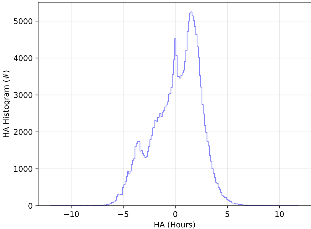
ddf_acor_sf10_lsf30_lsr50_v3.4_10yrs All sky g band: HA Histogram
