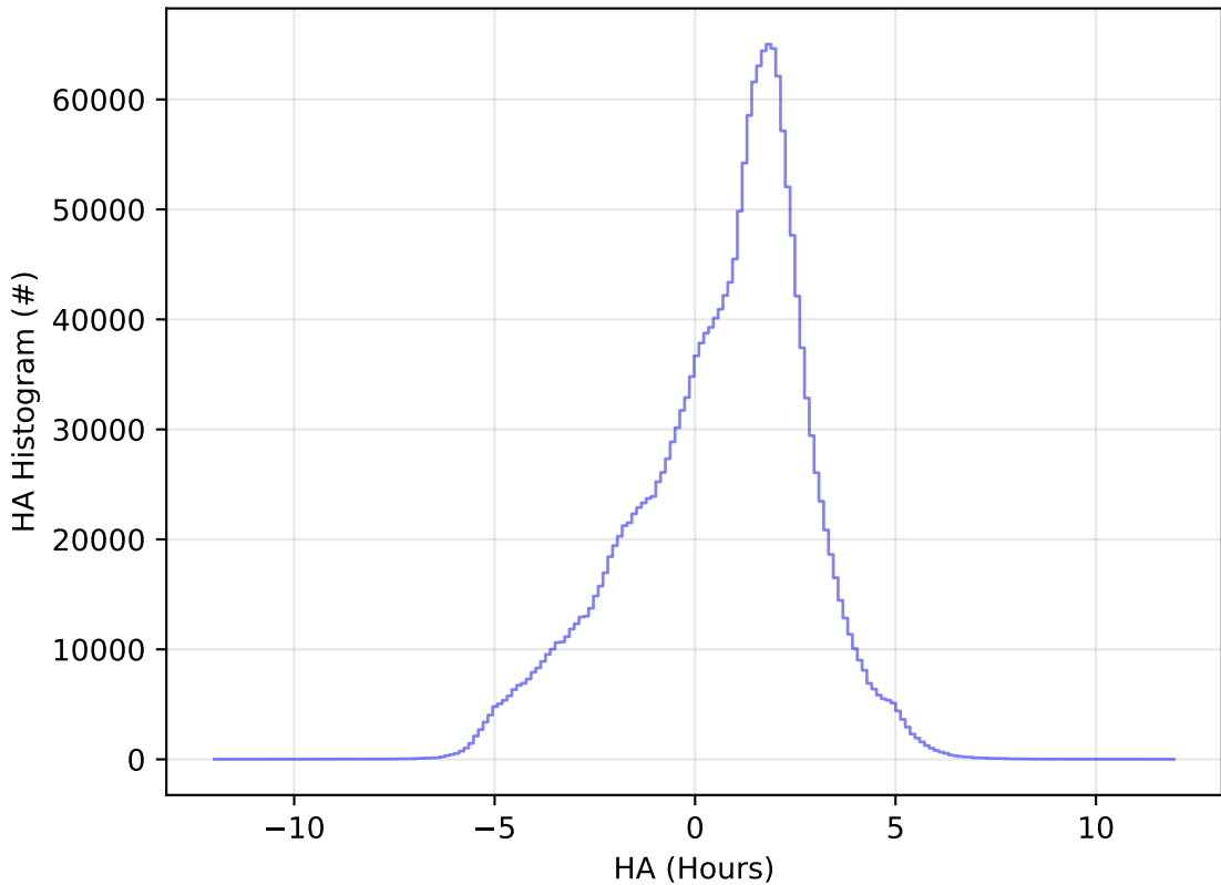
ddf_acor_sf10_lsf30_lsr50_v3.4_10yrs All sky all bands: HA Histogram
