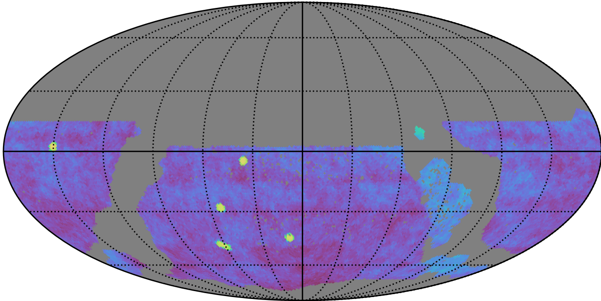
ddf_acor_sf10_lsf30_lsr50_v3.4_10yrs gri WFD: Fraction of visits in pairs (10-60 min)
