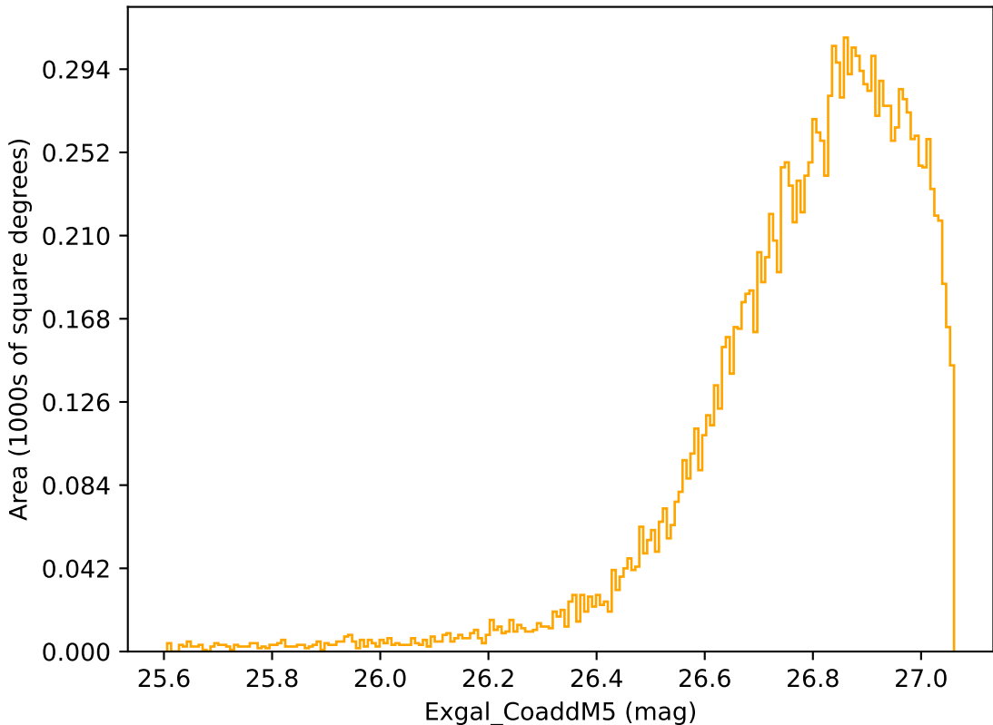
ddf_acor_sf10_lsf30_lsr50_v3.4_10yrs WFD r band: Exgal_CoaddM5
