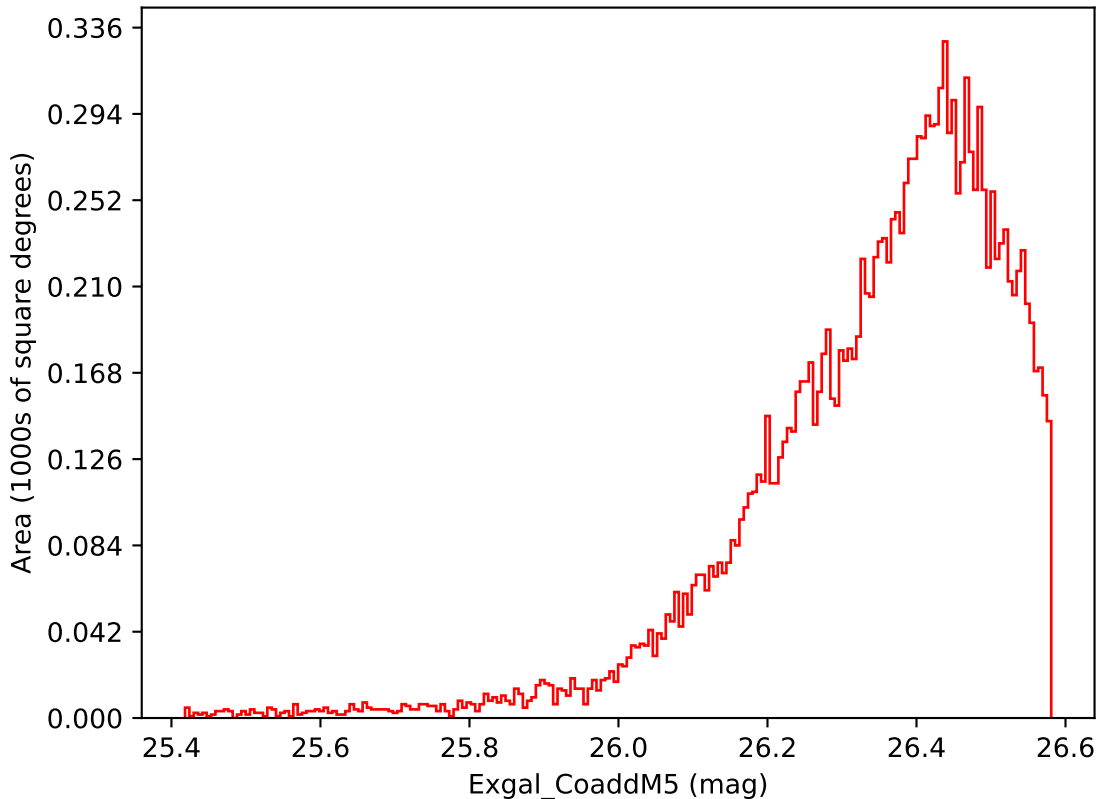
ddf_acor_sf10_lsf30_lsr50_v3.4_10yrs WFD i band: Exgal_CoaddM5
