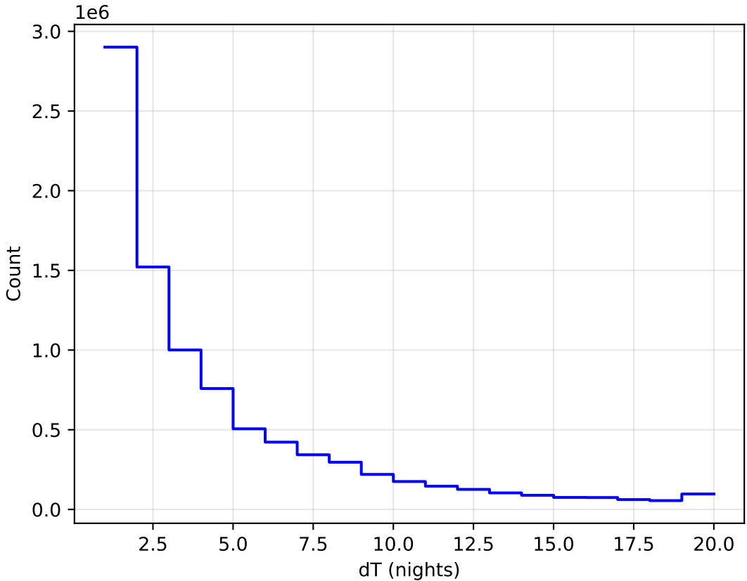
ddf_acor_sf10_lsf30_lsr50_v3.4_10yrs All sky all bands: DeltaNight Histogram
