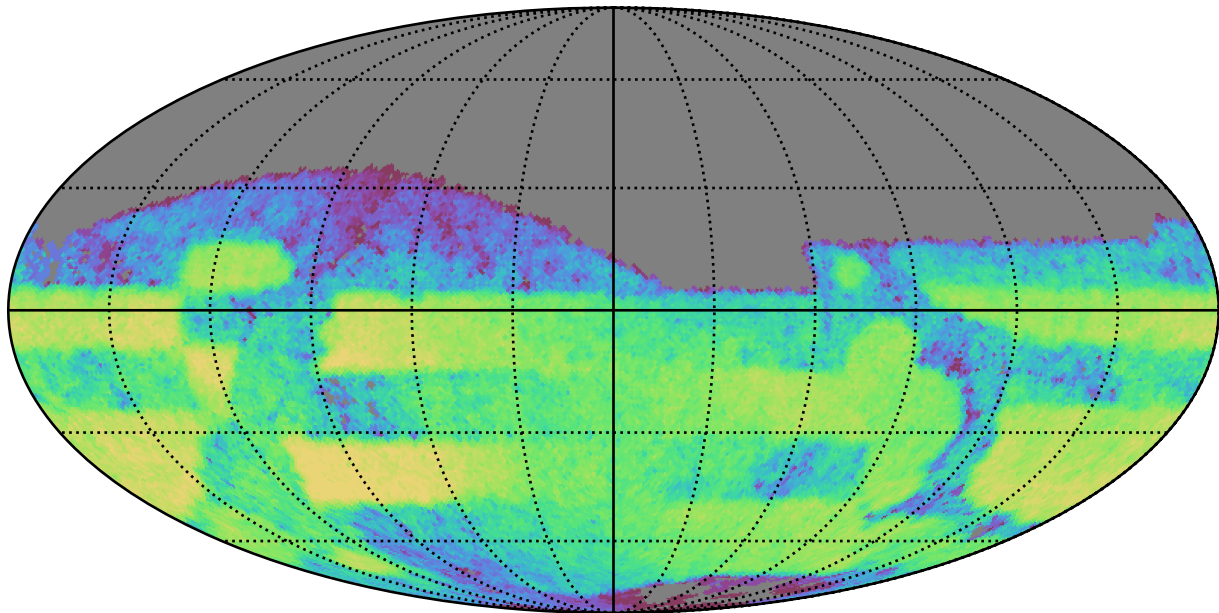
ddf_acor_sf10_lsf30_lsr50_v3.4_10yrs Yr 3-4 r band: CoaddM5
