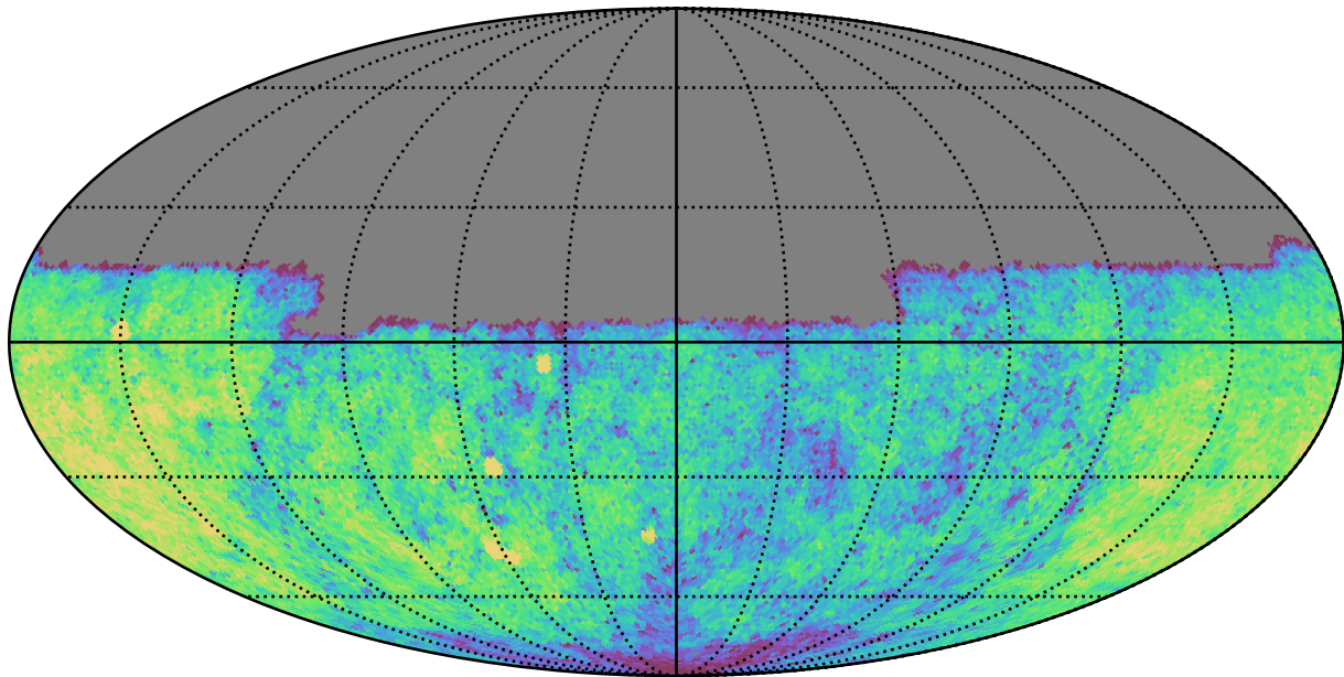
ddf_acor_sf10_lsf30_lsr50_v3.4_10yrs Yr 1 u band: CoaddM5
