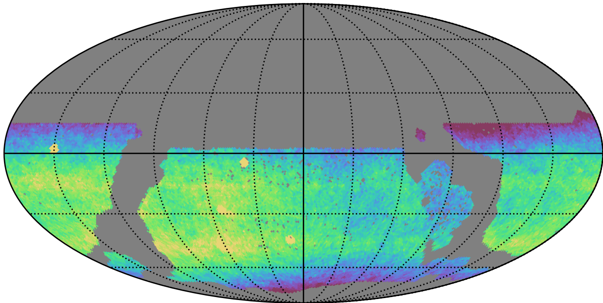
ddf_acor_sf10_lsf30_lsr50_v3.4_10yrs WFD z band: CoaddM5
