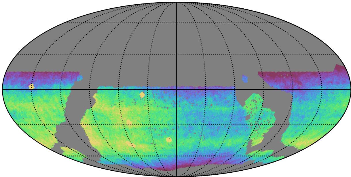
ddf_acor_sf10_lsf30_lsr50_v3.4_10yrs WFD r band: CoaddM5
