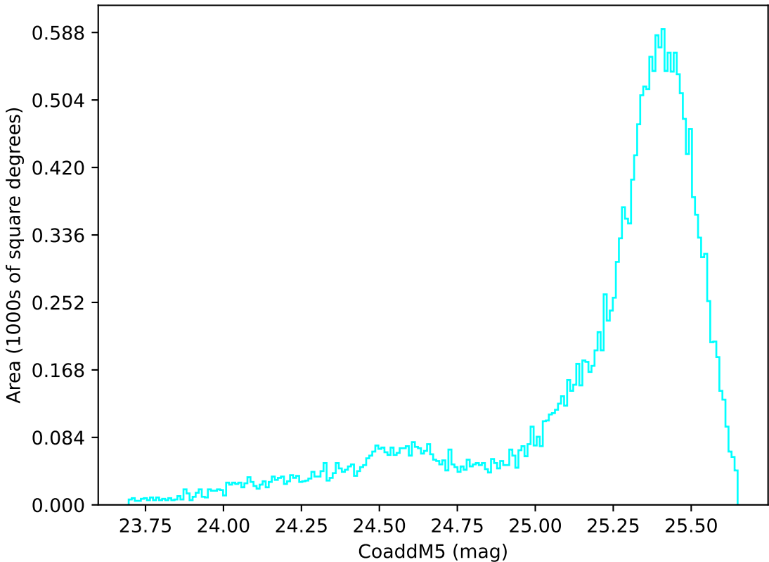
ddf_acor_sf10_lsf30_lsr50_v3.4_10yrs All sky u band: CoaddM5
