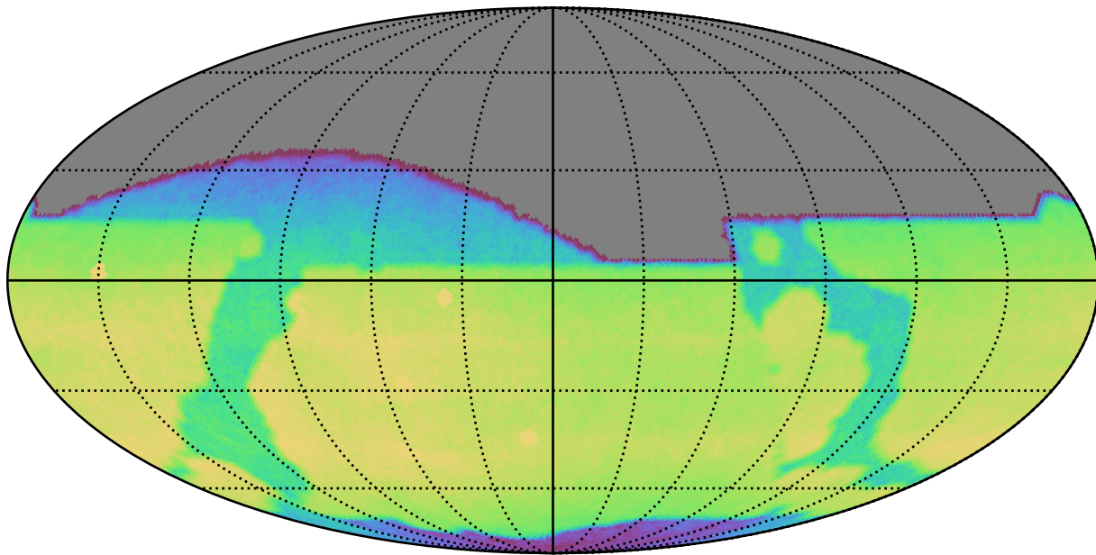
ddf_acor_sf10_lsf30_lsr50_v3.4_10yrs All sky r band: CoaddM5
