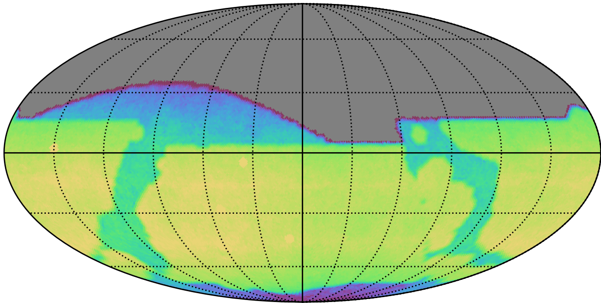
ddf_acor_sf10_lsf30_lsr50_v3.4_10yrs All sky i band: CoaddM5
