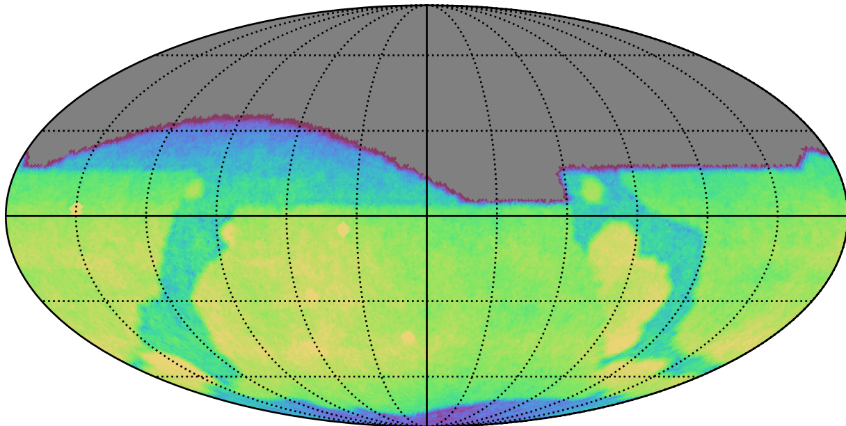
ddf_acor_sf10_lsf30_lsr50_v3.4_10yrs All sky g band: CoaddM5
