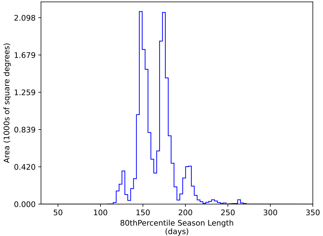
ddf_acor_sf10_lsf30_lsr50_v3.4_10yrs WFD y band: 80thPercentile Season Length
