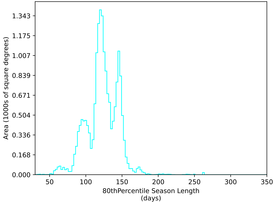
ddf_acor_sf10_lsf30_lsr50_v3.4_10yrs WFD u band: 80thPercentile Season Length
