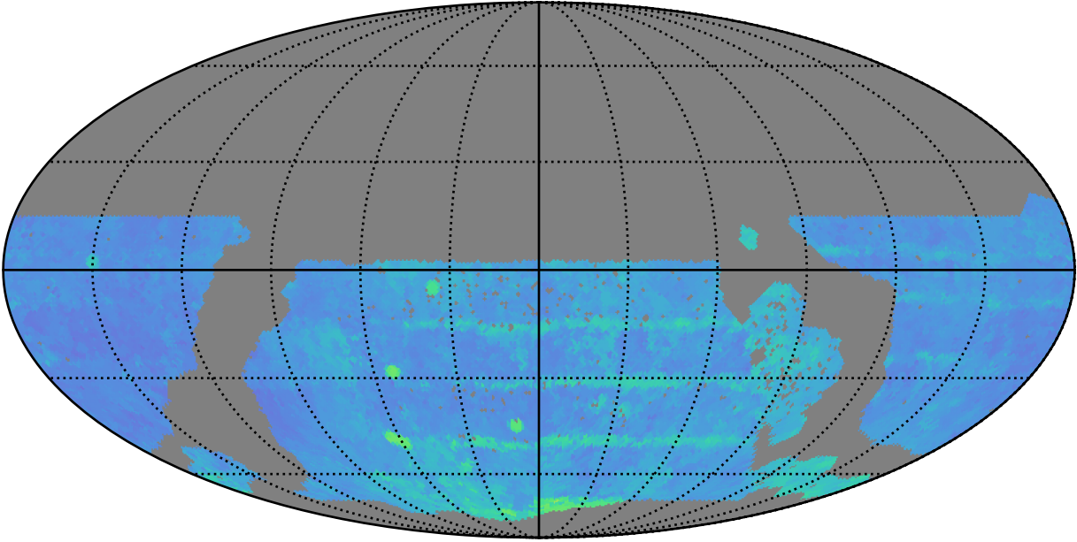
ddf_acor_sf10_lsf30_lsr50_v3.4_10yrs WFD i band: 80thPercentile Season Length
