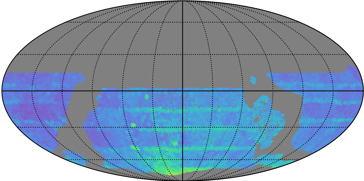
ddf_acor_sf10_lsf30_lsr50_v3.4_10yrs WFD all bands: 80thPercentile Season Length
