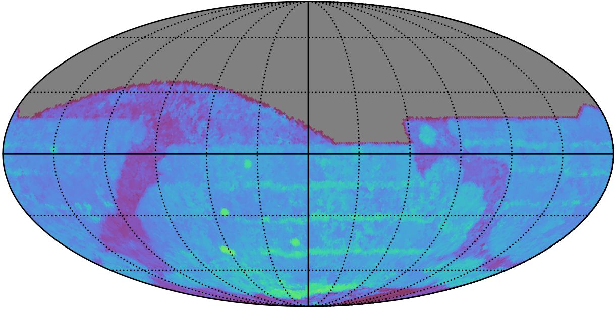
ddf_acor_sf10_lsf30_lsr50_v3.4_10yrs All sky z band: 80thPercentile Season Length
