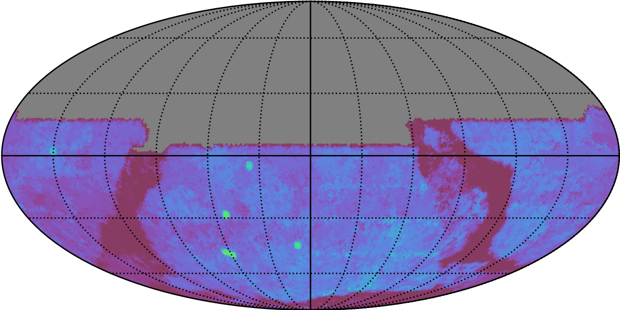
ddf_acor_sf10_lsf30_lsr50_v3.4_10yrs All sky u band: 80thPercentile Season Length
