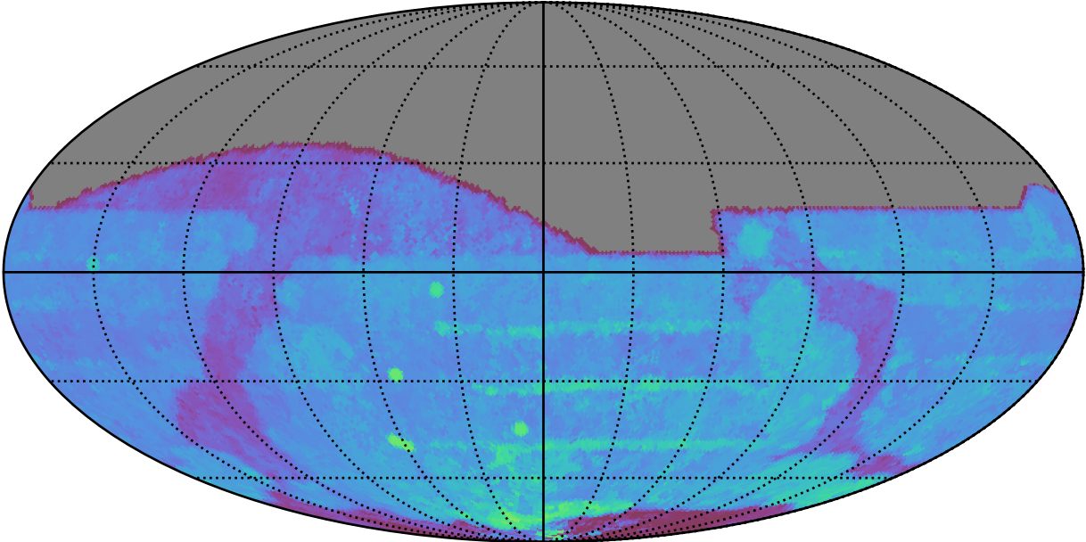
ddf_acor_sf10_lsf30_lsr50_v3.4_10yrs All sky r band: 80thPercentile Season Length
