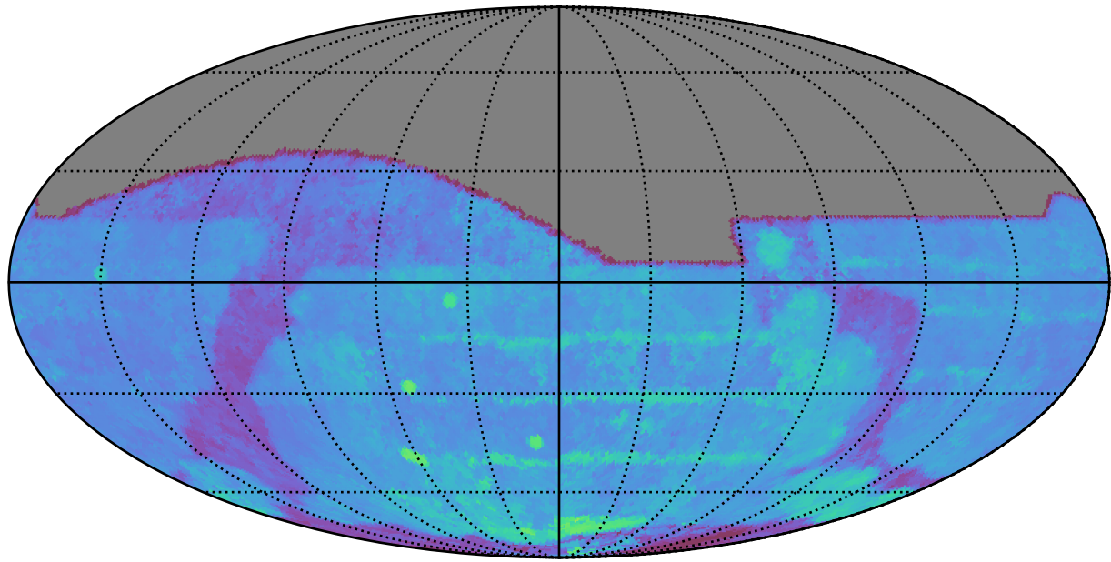
ddf_acor_sf10_lsf30_lsr50_v3.4_10yrs All sky i band: 80thPercentile Season Length
