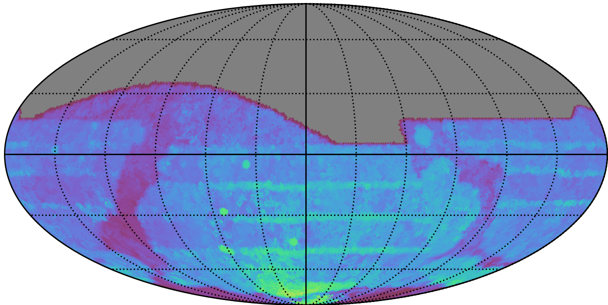
ddf_acor_sf10_lsf30_lsr50_v3.4_10yrs All sky all bands: 80thPercentile Season Length
