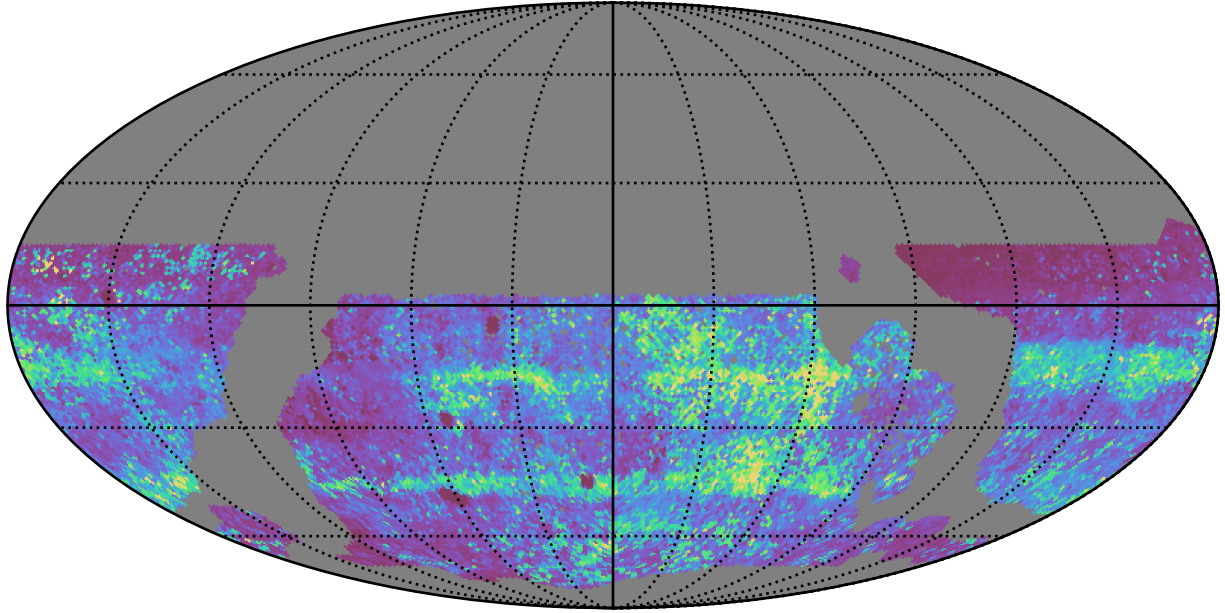
ddf_acor_sf10_lsf30_lsr50_v3.4_10yrs WFD zy bands: 75th Percentile Intranight Timespan
