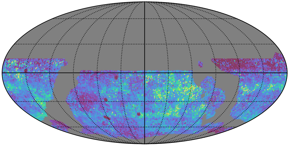
ddf_acor_sf10_lsf30_lsr50_v3.4_10yrs WFD y band: 75th Percentile Intranight Timespan
