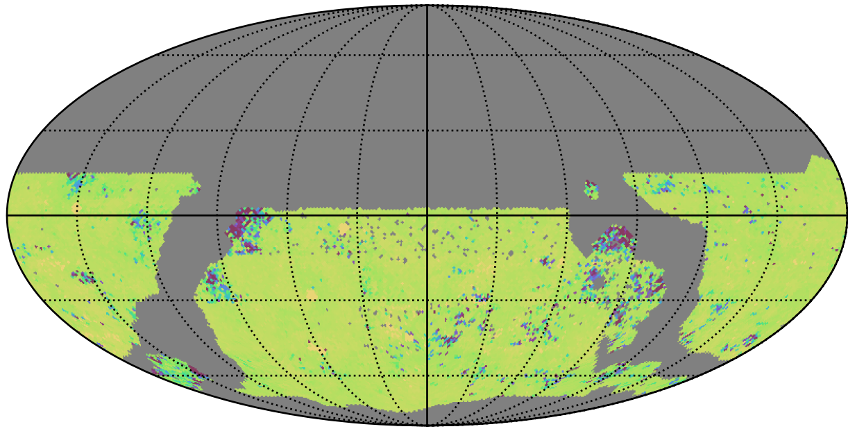
ddf_acor_sf10_lsf30_lsr50_v3.4_10yrs WFD ug bands: 75th Percentile Intranight Timespan
