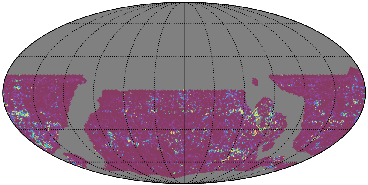
ddf_acor_sf10_lsf30_lsr50_v3.4_10yrs WFD u band: 75th Percentile Intranight Timespan
