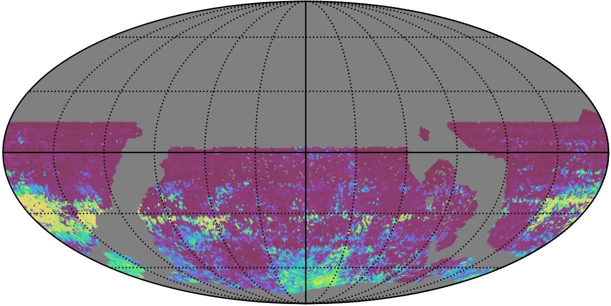
ddf_acor_sf10_lsf30_lsr50_v3.4_10yrs WFD r band: 75th Percentile Intranight Timespan
