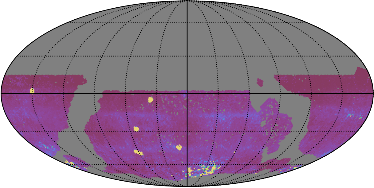
ddf_acor_sf10_lsf30_lsr50_v3.4_10yrs WFD iz bands: 75th Percentile Intranight Timespan
