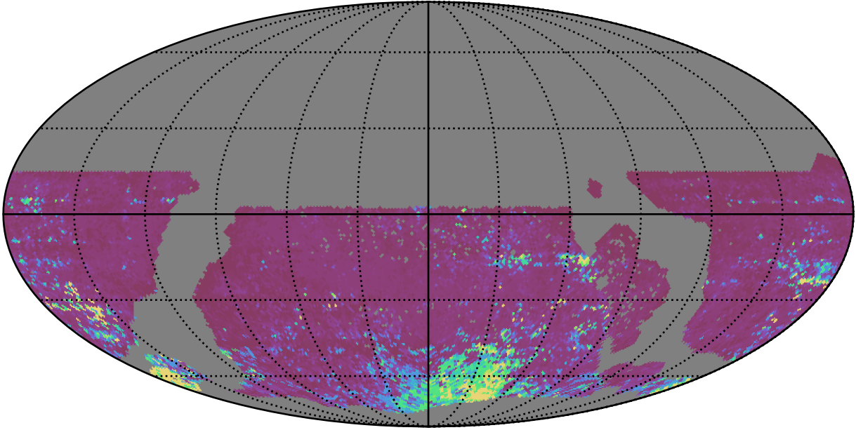
ddf_acor_sf10_lsf30_lsr50_v3.4_10yrs WFD i band: 75th Percentile Intranight Timespan
