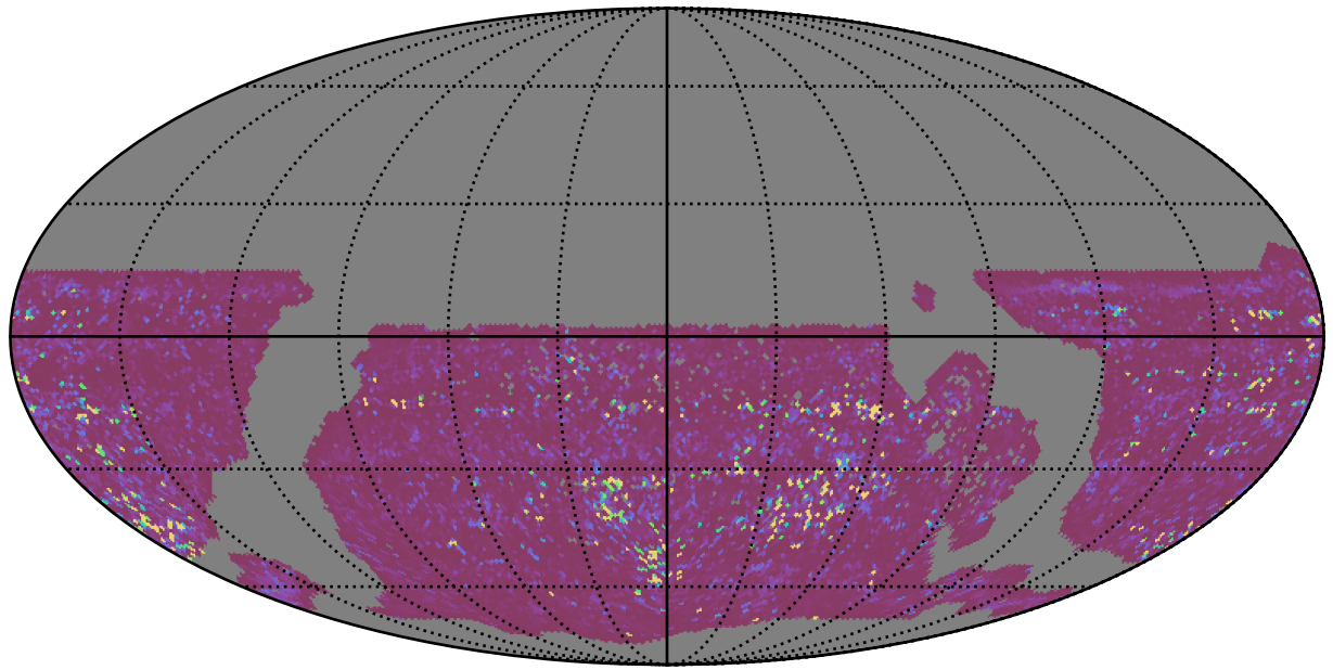
ddf_acor_sf10_lsf30_lsr50_v3.4_10yrs WFD g band: 75th Percentile Intranight Timespan
