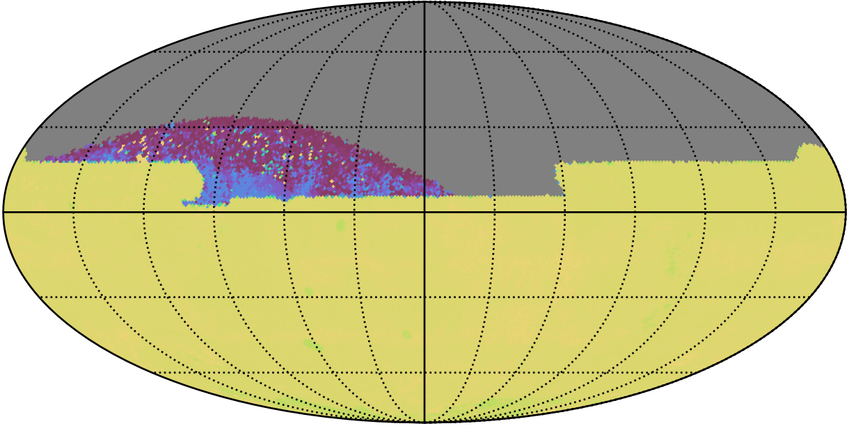
ddf_acor_sf10_lsf30_lsr50_v3.4_10yrs All sky zy bands: 75th Percentile Intranight Timespan
