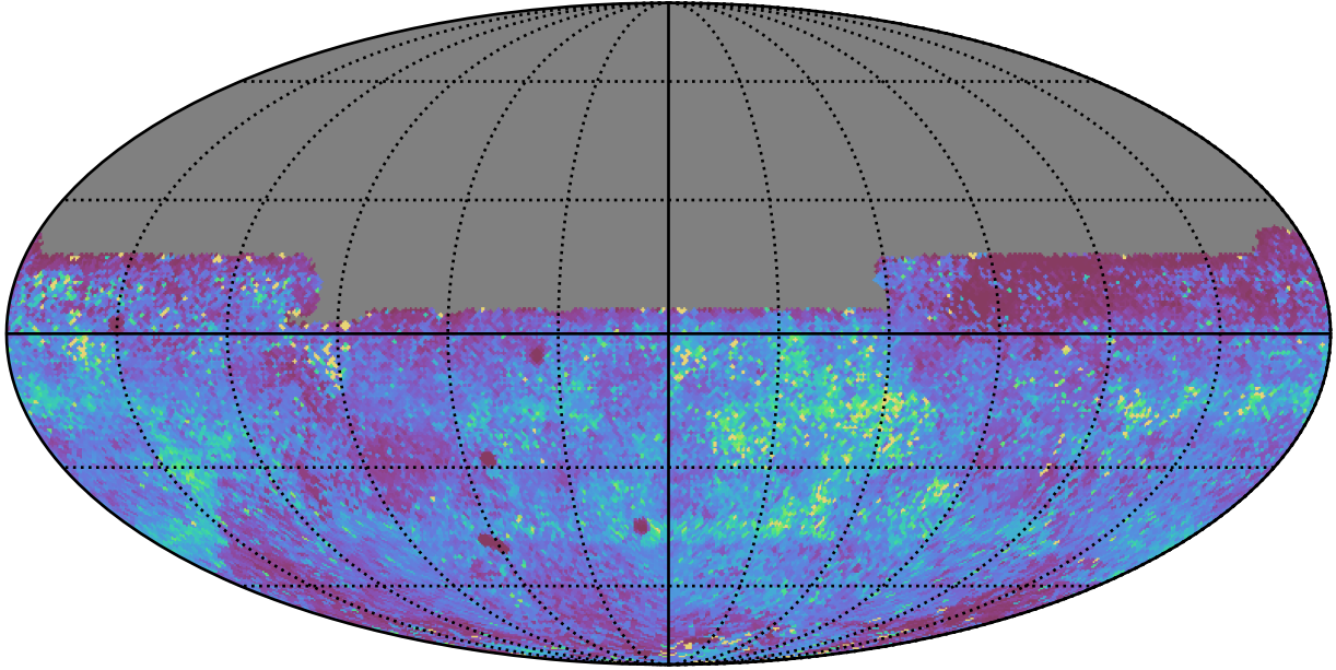
ddf_acor_sf10_lsf30_lsr50_v3.4_10yrs All sky y band: 75th Percentile Intranight Timespan
