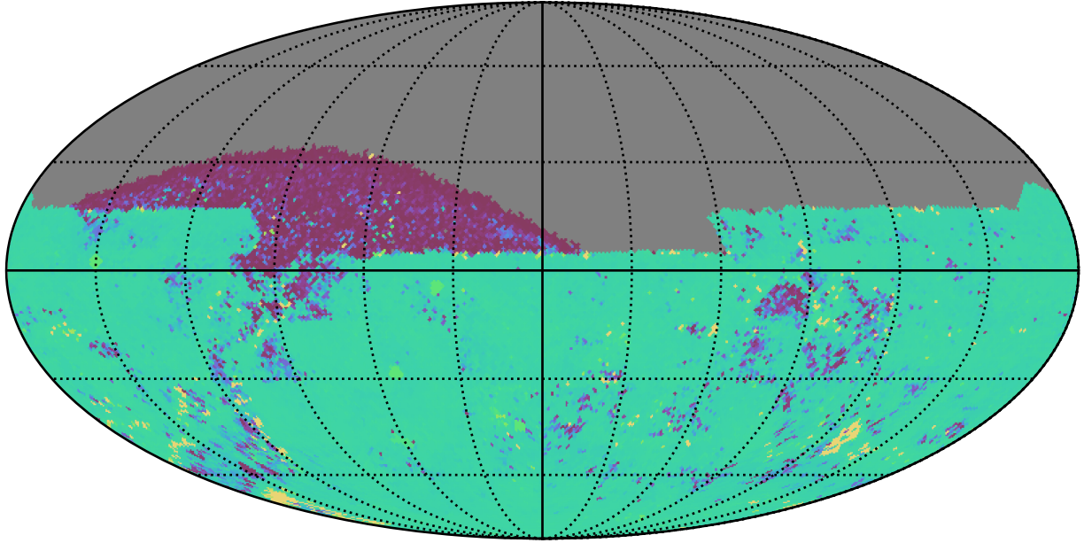
ddf_acor_sf10_lsf30_lsr50_v3.4_10yrs All sky ug bands: 75th Percentile Intranight Timespan
