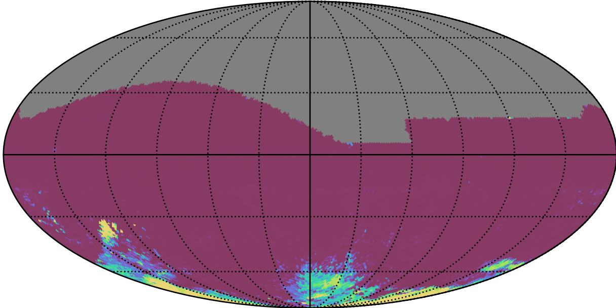
ddf_acor_sf10_lsf30_lsr50_v3.4_10yrs All sky ri bands: 75th Percentile Intranight Timespan
