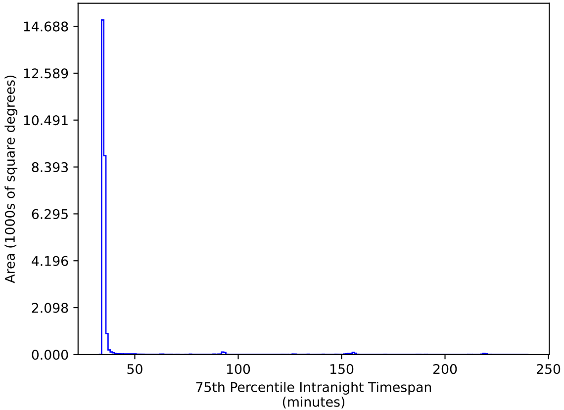
ddf_acor_sf10_lsf30_lsr50_v3.4_10yrs All sky ri bands: 75th Percentile Intranight Timespan
