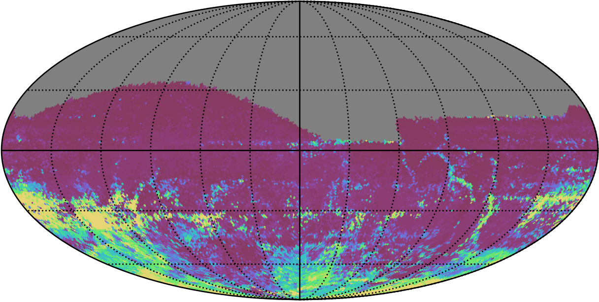
ddf_acor_sf10_ls30_lsr50_v3.4_10yrs All sky r band: 75th Percentile Intranight Timespan
