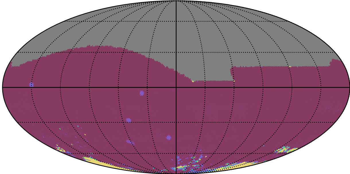
ddf_acor_sf10_lsf30_lsr50_v3.4_10yrs All sky iz bands: 75th Percentile Intranight Timespan
