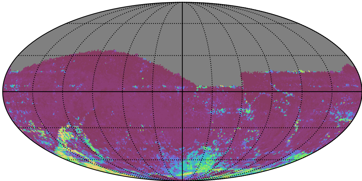
ddf_acor_sf10_lsf30_lsr50_v3.4_10yrs All sky i band: 75th Percentile Intranight Timespan
