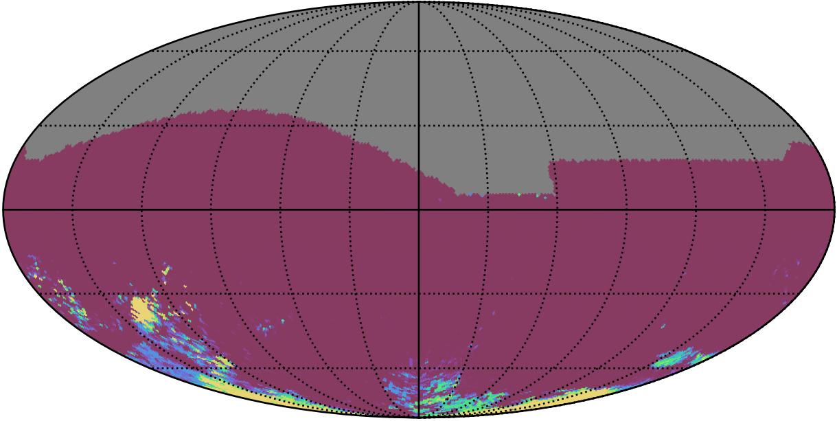
ddf_acor_sf10_lsf30_lsr50_v3.4_10yrs All sky gr bands: 75th Percentile Intranight Timespan
